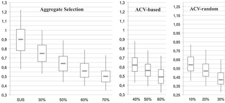
Fig. 5 ACV_{scaled} of the three selection strategies with different p_0 -values and TS = 10
