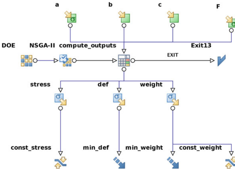
Fig. 7 H-beam: optimization workflow. From top to bottom: input variables ( a , b , c , F ), DOE, optimizer and calculator nodes, output variables \sigma , \delta , W (respectively denoted by stress , def , weight ), constraints on \sigma^{99.999} and W ( const_stress , const_weight ), and objectives on \delta^{99.999} and W ( min_def , min_weight )
